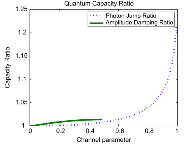
Fig. 1. Ratio of the true quantum capacity to the symmetric coherent information as a function of the channel parameter for both the amplitude damping channel and the photon-detected jump channel (see Appendix B for definitions of these channels). Observe that the ratio is close to 1 for many values of the channel parameters.
