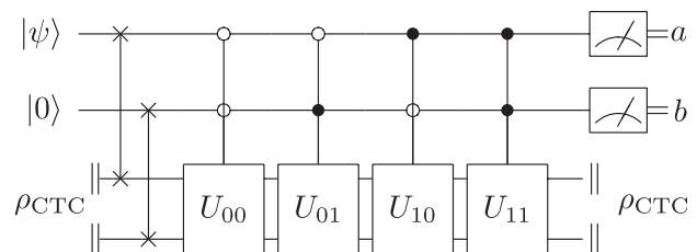
FIG. 2. The above circuit can perfectly distinguish the BB84 states |0\rangle, |1\rangle, |+\rangle , and |-\rangle . The circuit uses the standard quantum circuit notation from Ref. [14] and we define the unitaries U_{00}, U_{01}, U_{10} , and U_{11} in (3).
